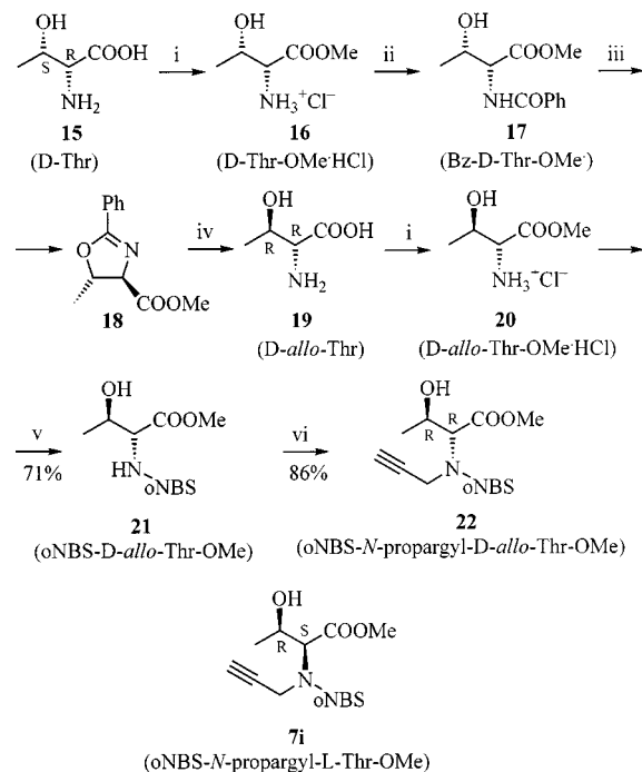
Scheme 2. Synthesis of o -NBS- N -allyl-L-Ser-OMe ( 7f ) and o -NBS- N -propargyl-L-Thr-OMe ( 7i ) and mechanism of the elimination to the corresponding acrylic derivatives 11 and 12
